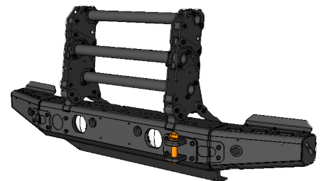
Two of 18 configurations of Pronghorn's Modular Front End System rendered in Cobalt CAD and 3D modelling software.
