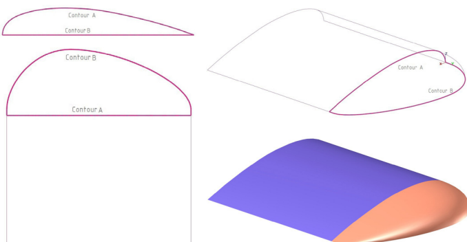
Spline created from two contours.
